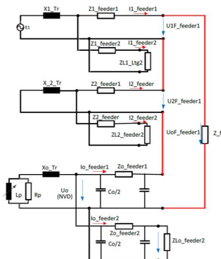
Figure 2 Symmetrical components situation with single phase to ground fault
