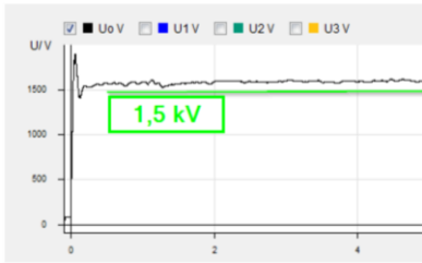
Figure 24 Detuning +40%, 5 kOhm fault impedance
