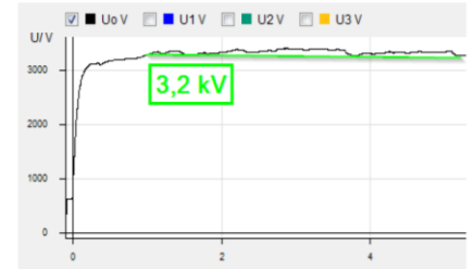
Figure 26 Detuning 0%, 5 kOhm fault impedance
