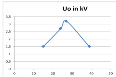
Figure 27 U_o vs. tuning position in A
