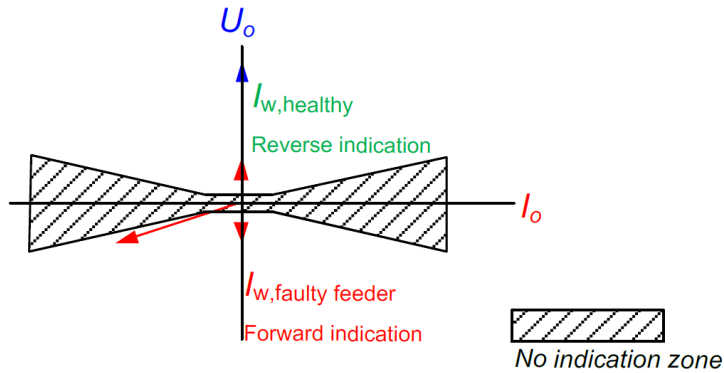
Figure 14 Indication zone for the wattmetric method
