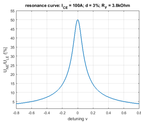
Figure 8 U_0 value for a 3.8 kOhm fault impedance vs. detuning of the ASC; network size 100 A
