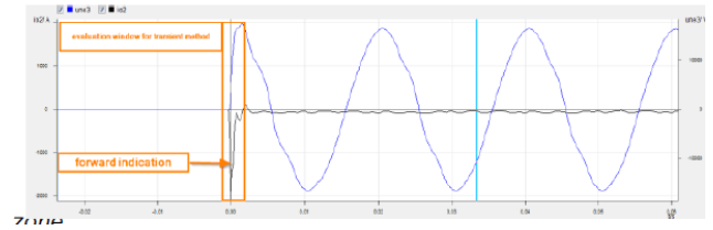
Figure 17 fault record transient stage; forward indication; low impedance fault
