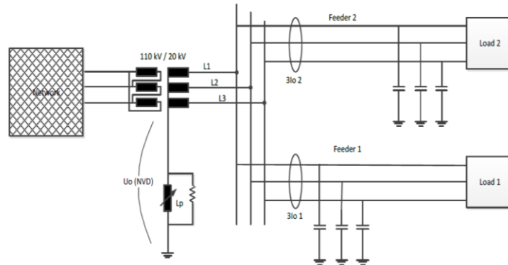
Figure 1 Arc suppression coil connected to the transformer neutral
