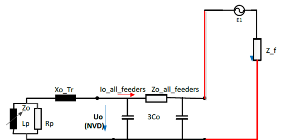
Figure 3 Simplified zero sequence equivalent diagram
