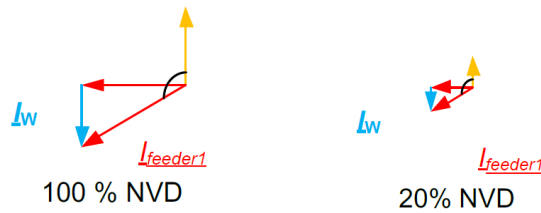
Figure 12 Vector diagram U_0 and I_0 ; low impedance fault vs. high impedance fault
