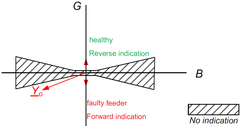
Figure 15 Admittance method indication zone
