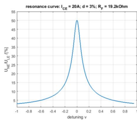
Figure 9 U_0 value for a 19.2 kOhm fault impedance vs. detuning of the ASC; network size is 20 A
