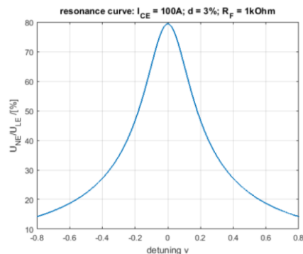
Figure 7 Changing the ASC tuning position during an earth fault with 1 kOhm fault impedance
