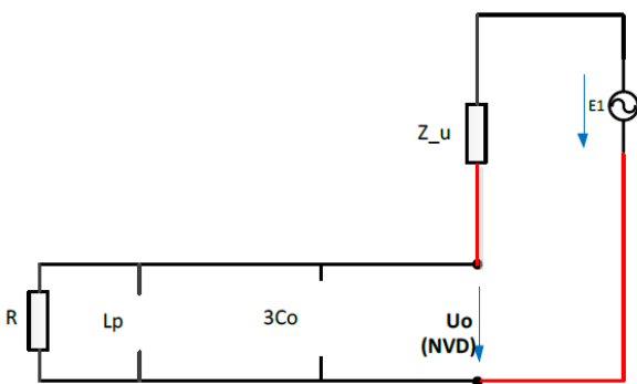
Figure 6 Equivalent diagram at the point of resonance
