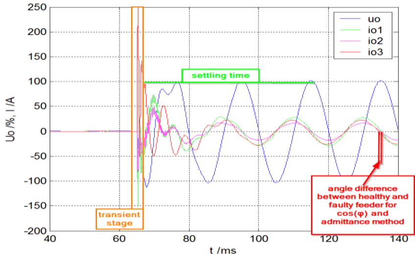
Figure 13 Very small angle difference for the wattmetric method between healthy and faulty (red) feeder
