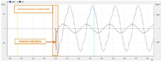
Figure 16 fault record for transient stage, reverse indication; low impedance fault
