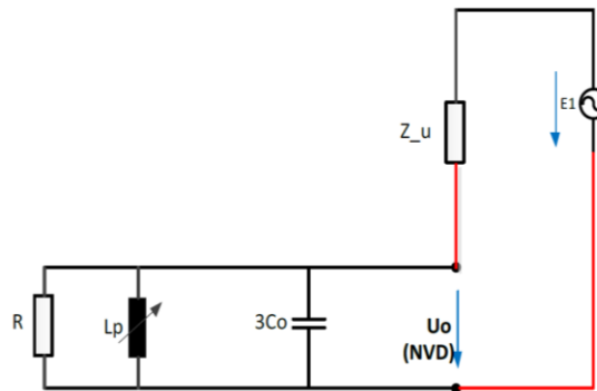
Figure 4 Equivalent zero sequence diagram for sensitivity estimation
