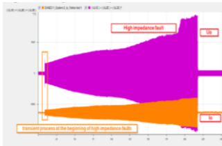
Figure 20 High impedance fault development for 200 s trigger
