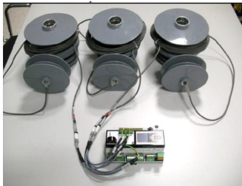
Figure 23 Overhead line combined sensor for phase voltage and current measurement connected to the EOR-3D (A. Eberle)
