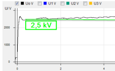
Figure 25 Detuning -10%, 5 kOhm fault impedance
